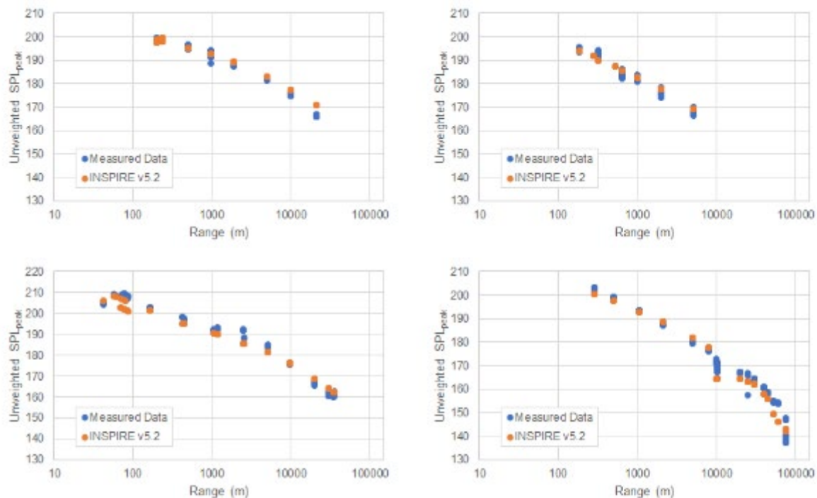
Figure 4-1 Comparison between example measured impact piling data (blue points) and modelled data using INSPIRE version 5.2 (orange points) 1
