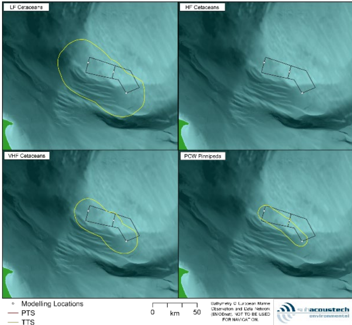
Figure A 1 Contour plots showing the in-combination impacts of concurrent installation of monopile foundations at three locations across DBS for marine mammals using the non-impulsive Southall et al. (2019) criteria assuming a fleeing animal
