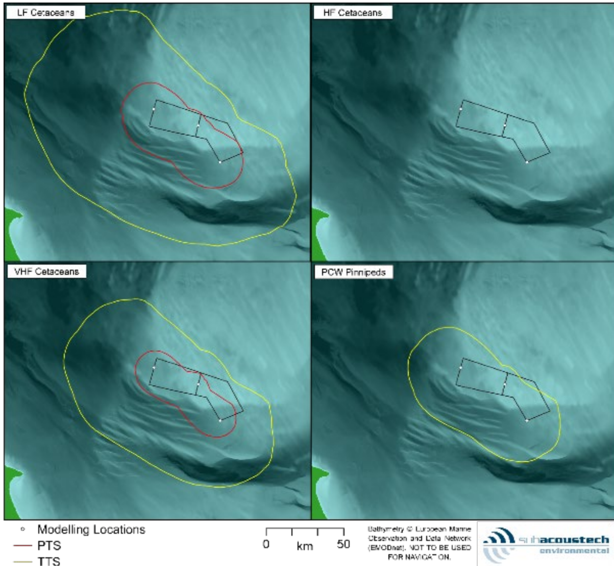
Figure 5-2 Contour plots showing the in-combination impacts of concurrent installation of monopile foundations at three locations across DBS for marine mammals using the impulsive Southall et al. (2019) criteria assuming a fleeing animal
