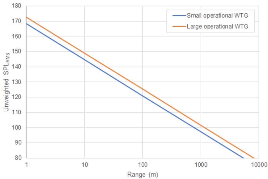
Figure 6-2 Predicted unweighted SPL_{RMS} from operational WTGs with power outputs of small and large turbine options using the calculation from Tougaard et al. (2020)
