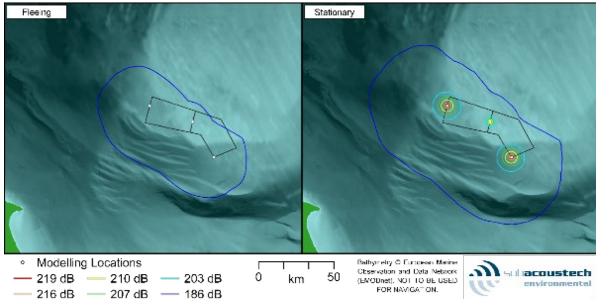
Figure 5-3 Contour plots showing the in-combination impacts of concurrent installation of monopile foundations at three locations across DBS for fish using the pile driving Popper et al. (2014) criteria assuming both a fleeing and stationary animal
