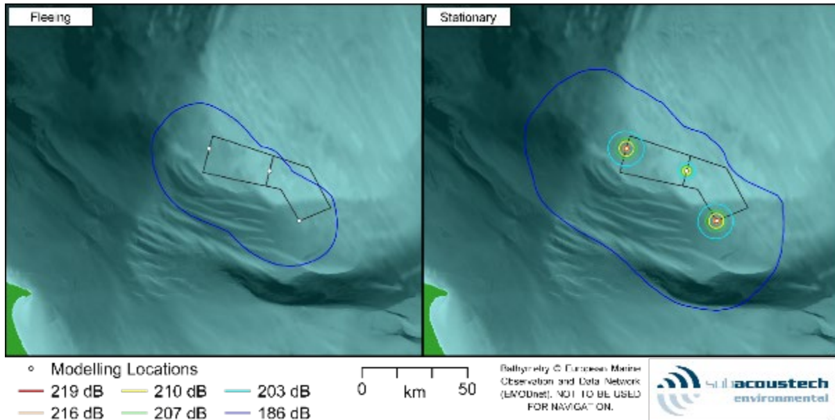
Figure 5-5 Contour plots showing the in-combination impacts of concurrent installation of pin pile jacket foundations at three locations across DBS for fish using the pile driving Popper et al. (2014) criteria assuming both a fleeing and stationary animal
