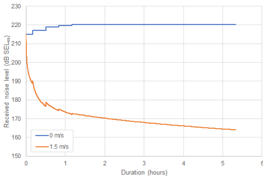
Figure 4-3 Received single-strike noise levels ( SEL_{ss} ) for receptors during the monopile foundation parameters at the Dogger Bank West: West location, assuming both a stationary and fleeing receptor starting at a location 1 m from the noise source
