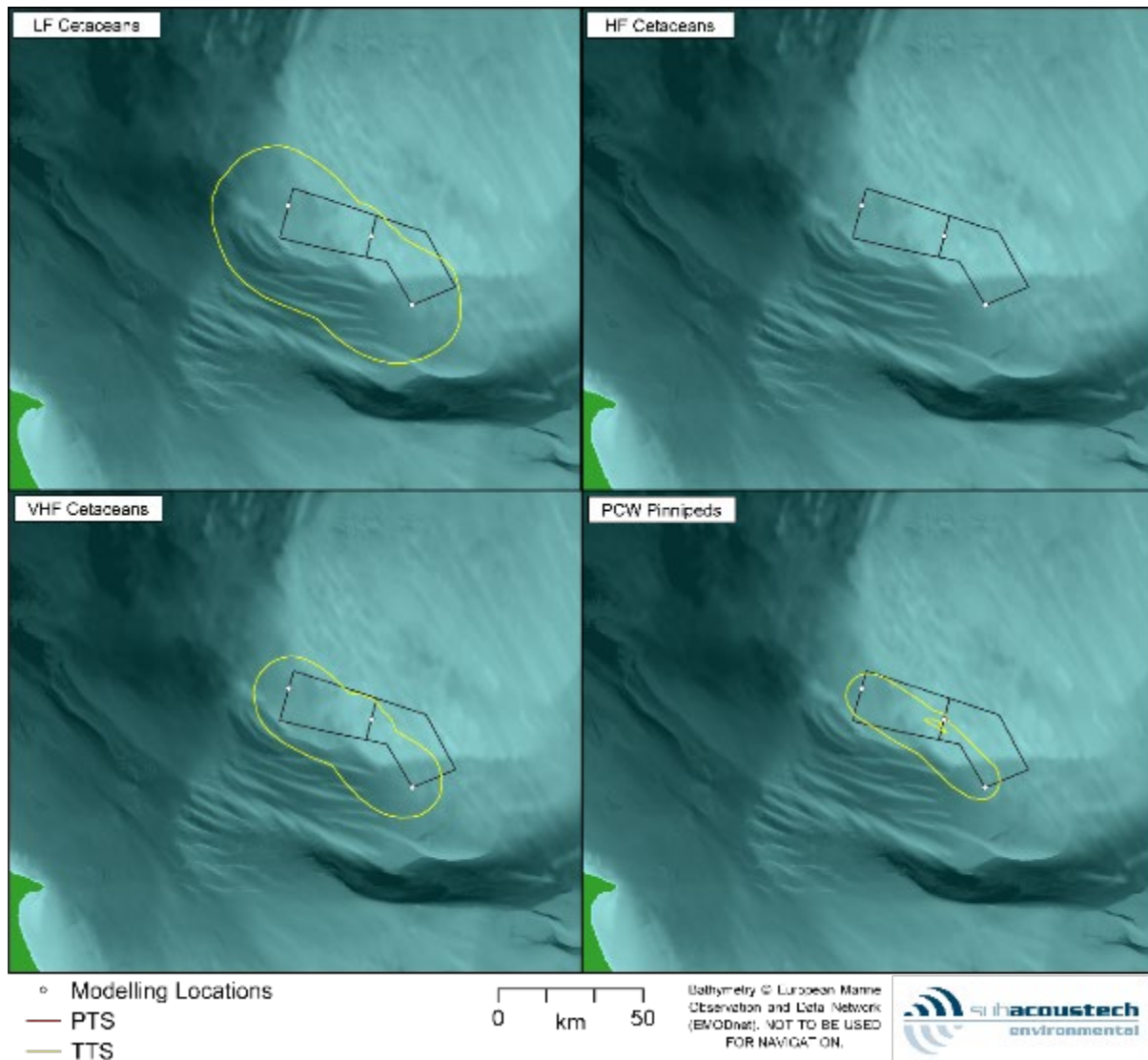
Figure A 2 Contour plots showing the in-combination impacts of concurrent installation of pin pile jacket foundations at three locations across DBS for marine mammals using the non-impulsive Southall et al. (2019) criteria assuming a fleeing animal
