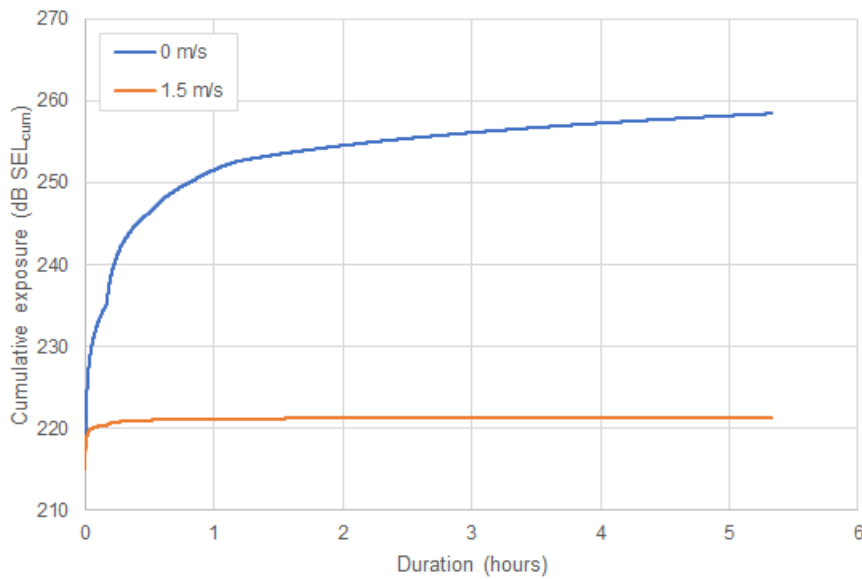
Figure 4-4 Cumulative received noise levels (SEL cum ) for receptors during monopile foundation parameters at the Dogger Bank West: West location, assuming both a stationary and fleeing receptor starting at a location 1 m from the noise source
