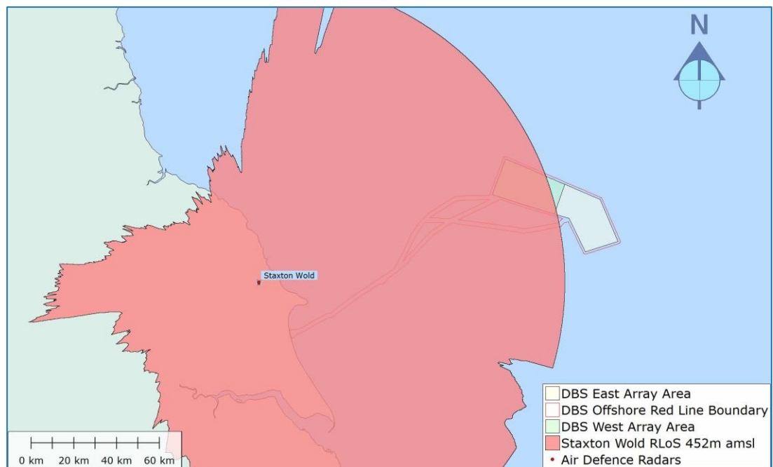
Figure 15: Staxton Wold RLoS 452m amsl
