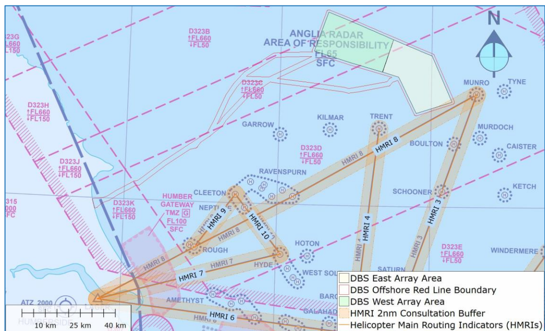
Figure 6: Helicopter Main Routing Indicators
