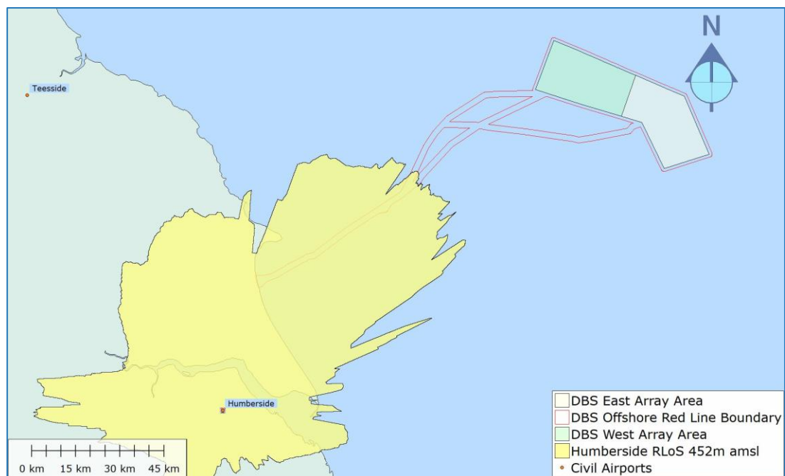
Figure 9: Humberside RLoS 452m amsl
