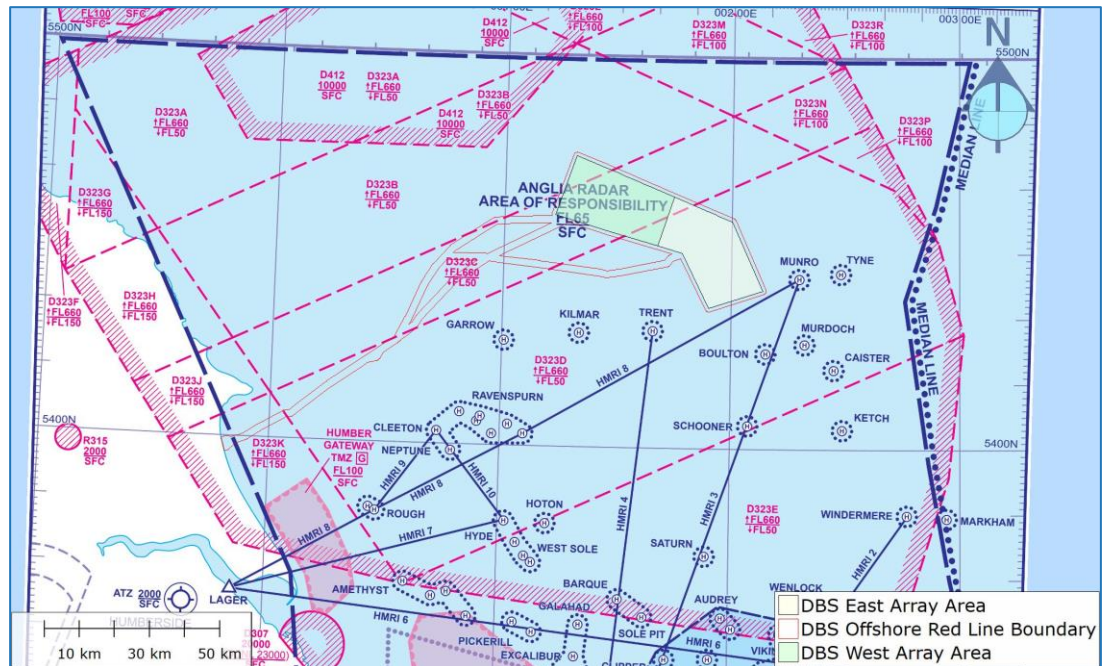
Figure 5: Anglia Radar Area of Responsibility
