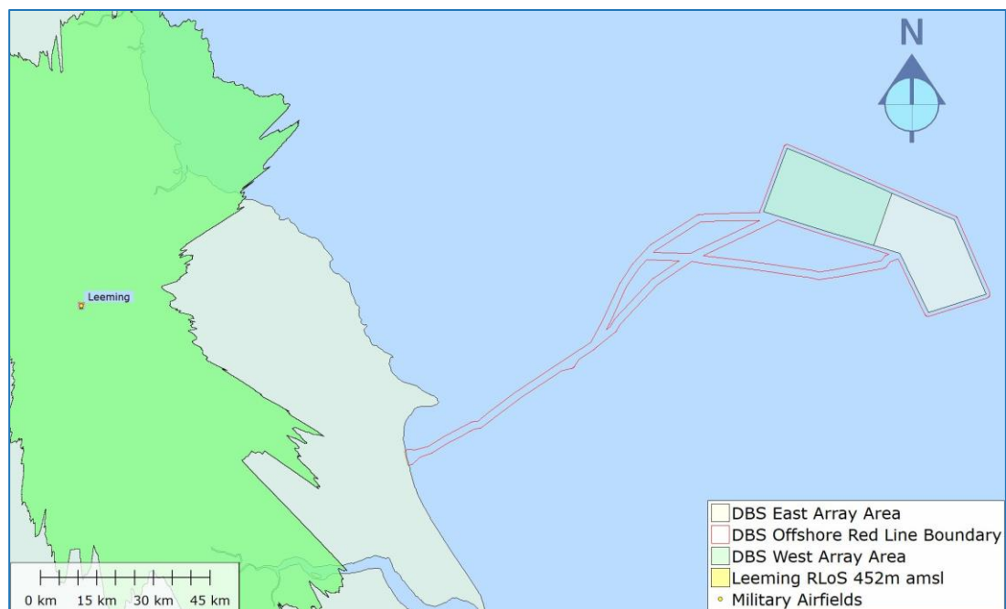
Figure 11: Leeming RLoS 400m amsl
