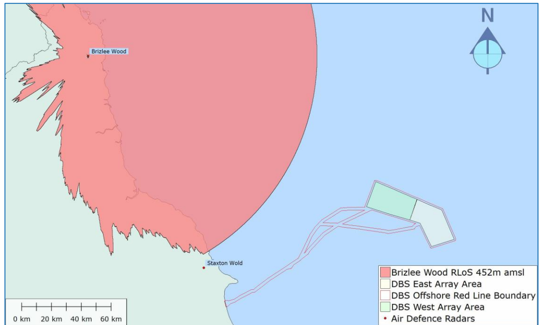
Figure 20: Brizlee Wood RLoS 452m amsl
