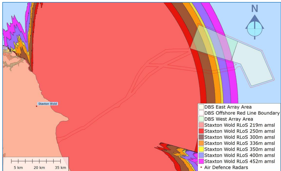
Figure 18: Staxton Wold RLoS coverages
