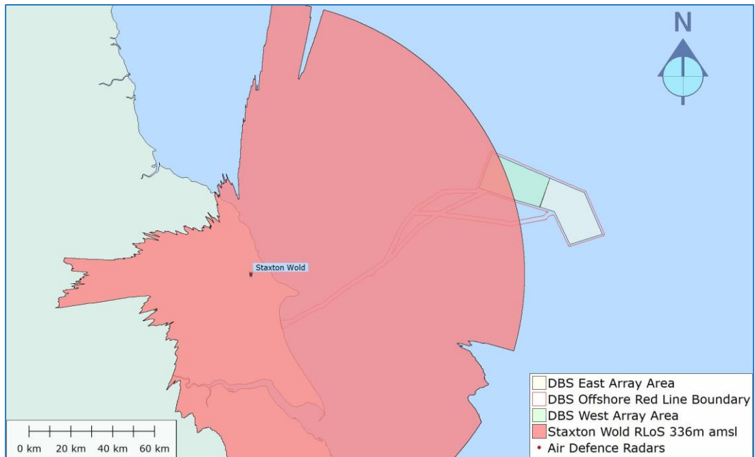
Figure 16: Staxton Wold RLoS 336m amsl
