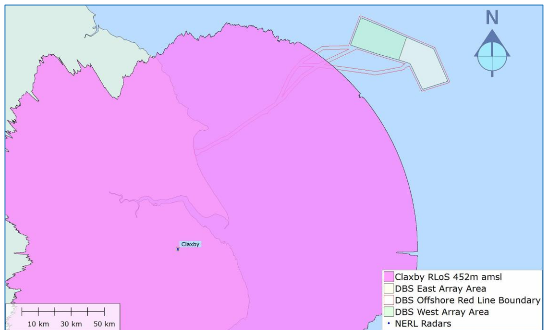
Figure 12: Claxby RLoS 452m amsl
