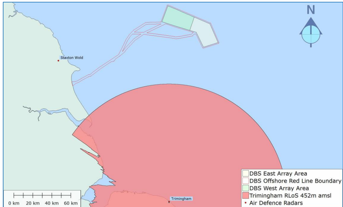
Figure 19: Trimingham RLoS 452m amsl
