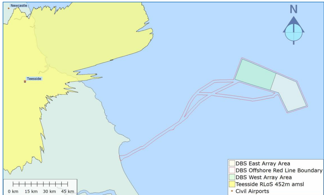
Figure 10: Teesside RLoS 452m amsl
