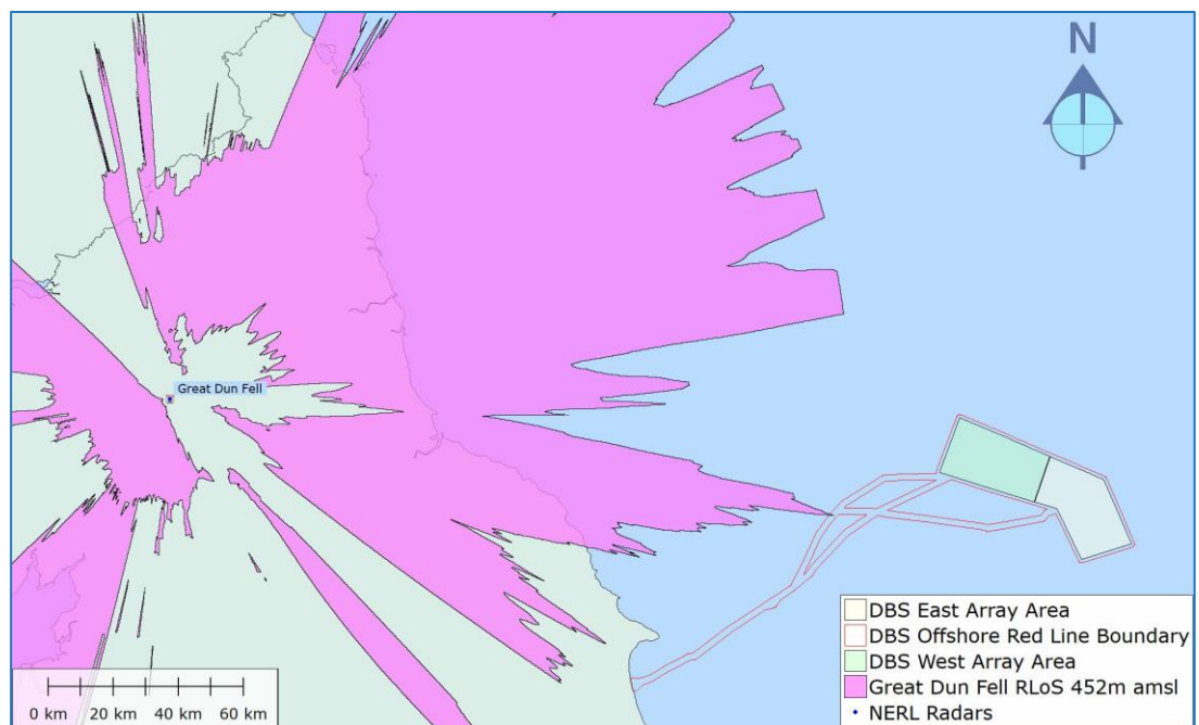
Figure 14: Great Dun Fell RLoS 452m amsl
