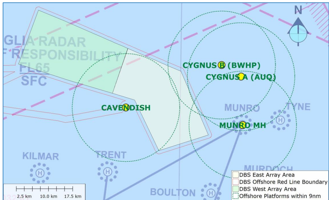
Figure 7: Offshore helidecks within 9nm of DBS array areas
