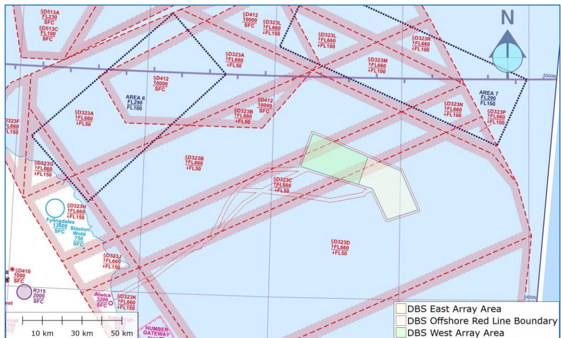
Figure 4: Southern MDA
