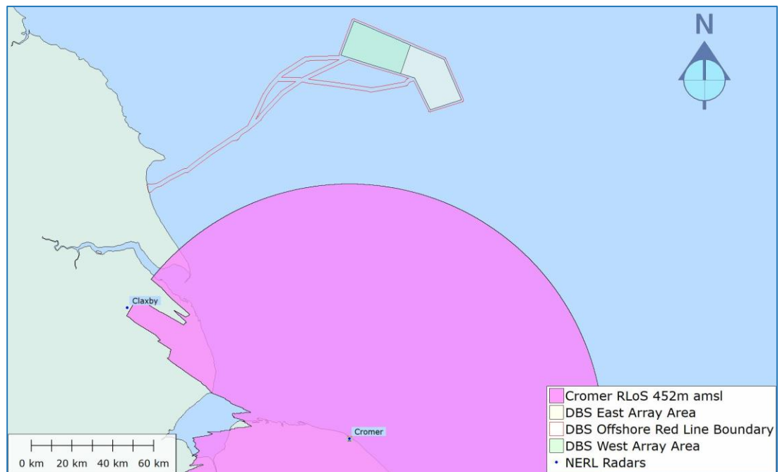
Figure 13: Cromer RLoS 452m amsl
