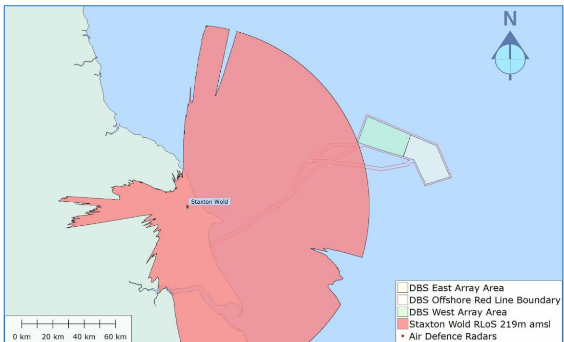
Figure 17: Staxton Wold RLoS 219m amsl
